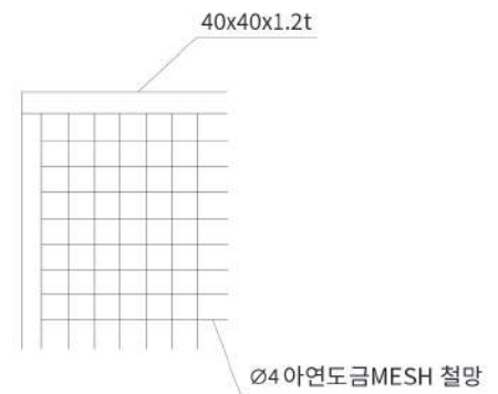
상세(Detailed Drawing)
