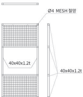
전면(Front View)
