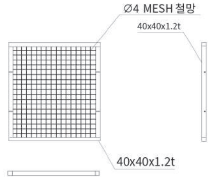
상세(Detailed Drawing)
