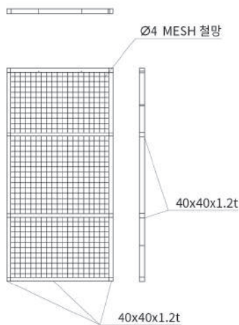
측면(Side View)
